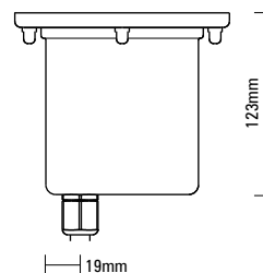
Bottom entry
