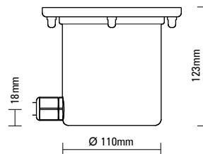
Side entry
