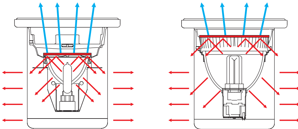
LS343 Metal Halide Configuration with Human Touch
