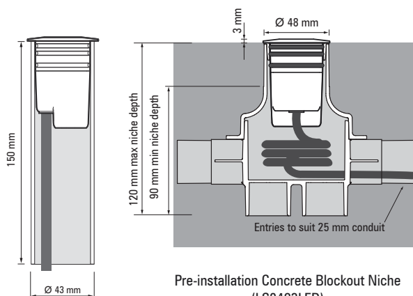
Installation Sleeve (LS9401LED)
